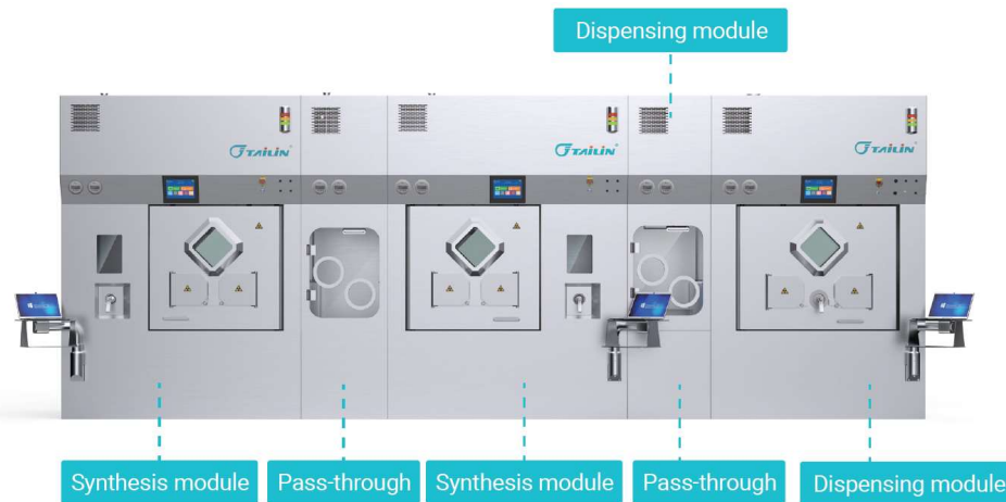
Hot Cell for Radiopharmaceutical Sterile Production
